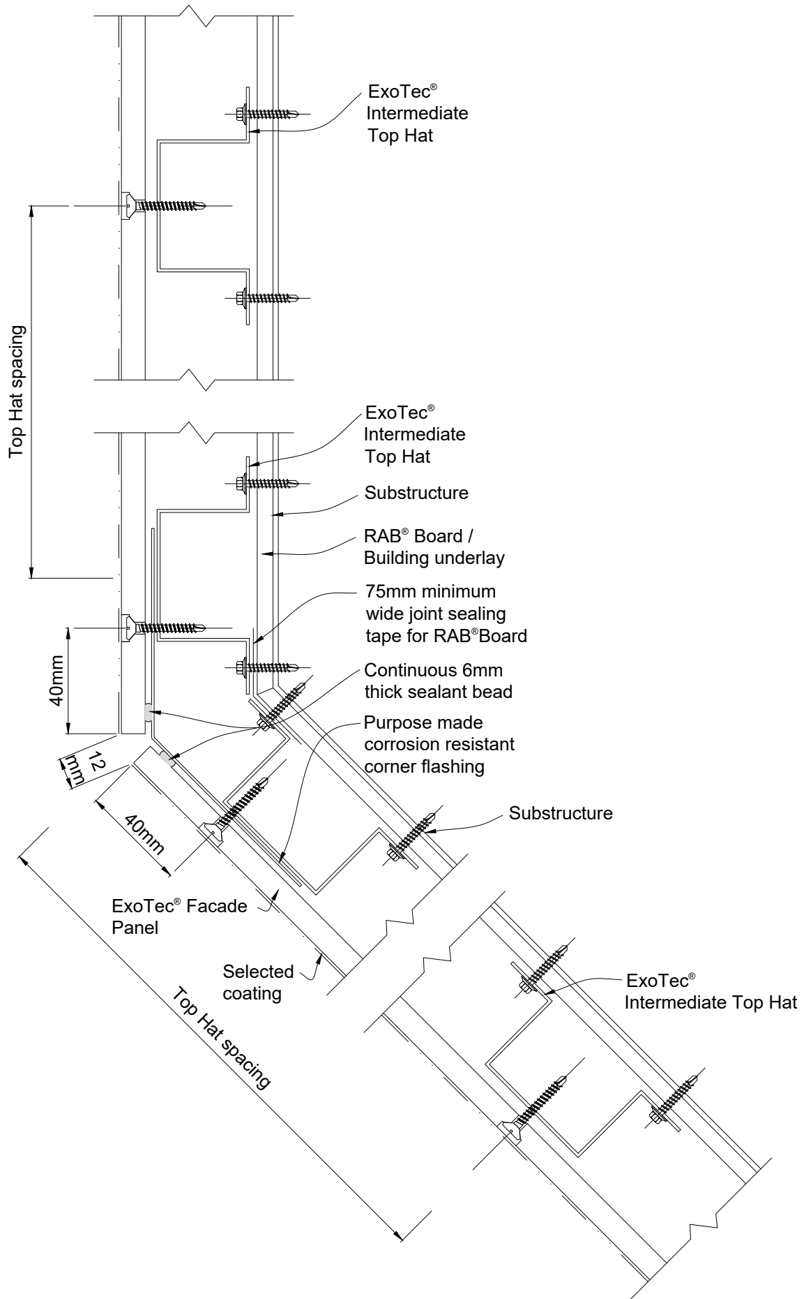
fig13 jhl_text_c_junc_cor-angl.dwg
